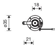
5.17633 fundamentanker
